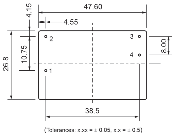
Pin View
