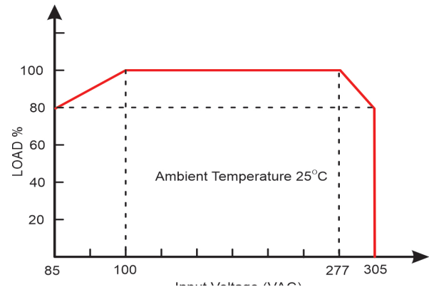
Input Voltage Derating Graph
