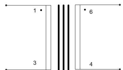
Electrical schematic
